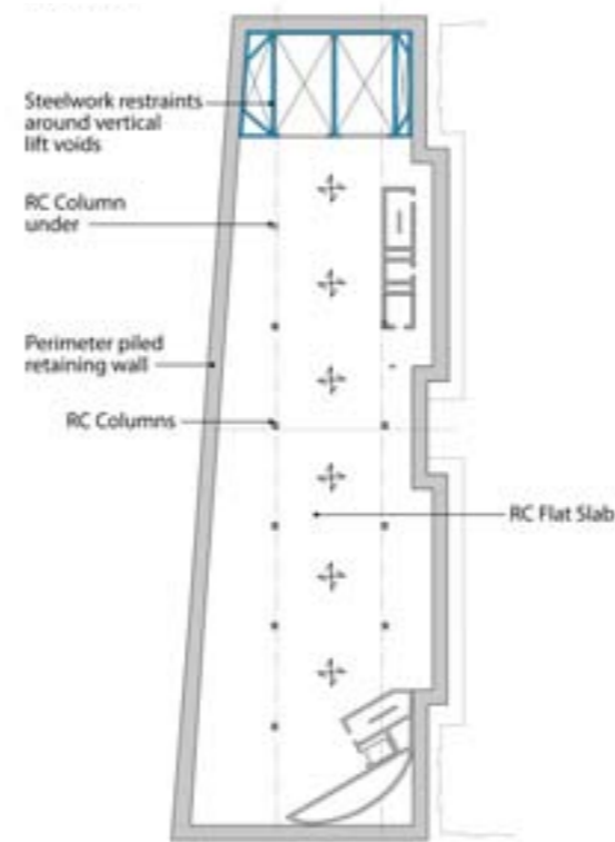
Seething Lane Garden Basement 2
