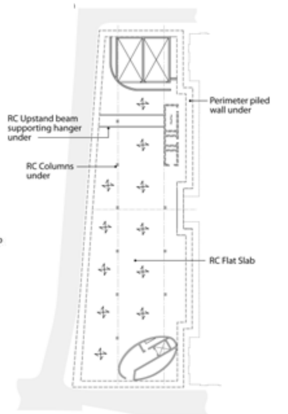
Seething Lane Garden Ground Floor
