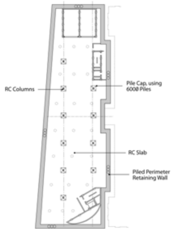
Seething Lane Garden Basement 4
