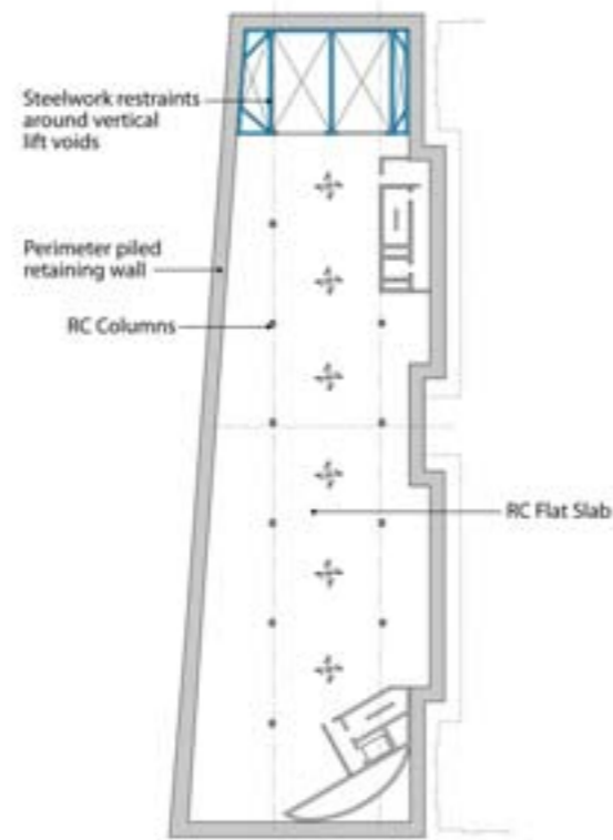
Seething Lane Garden Basement 3
