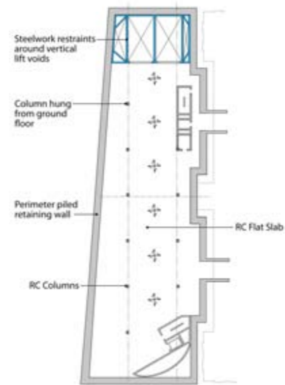
Seething Lane Garden Basement 1
